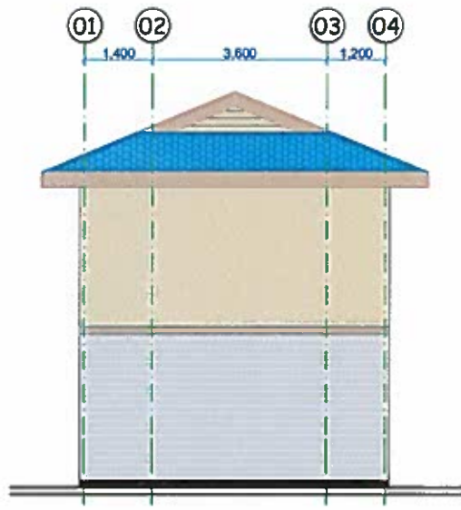
ELEVATION 03
